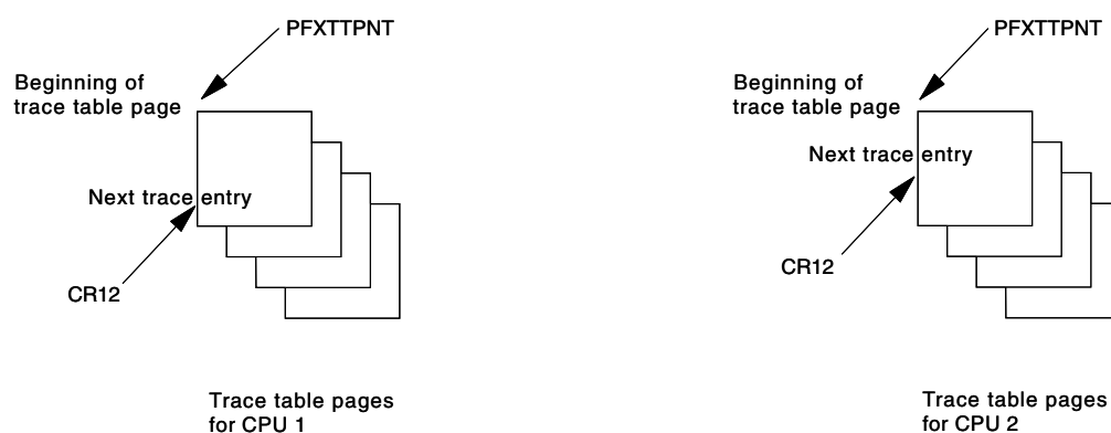
Figure 2. Trace Table Pages for Each Processor
