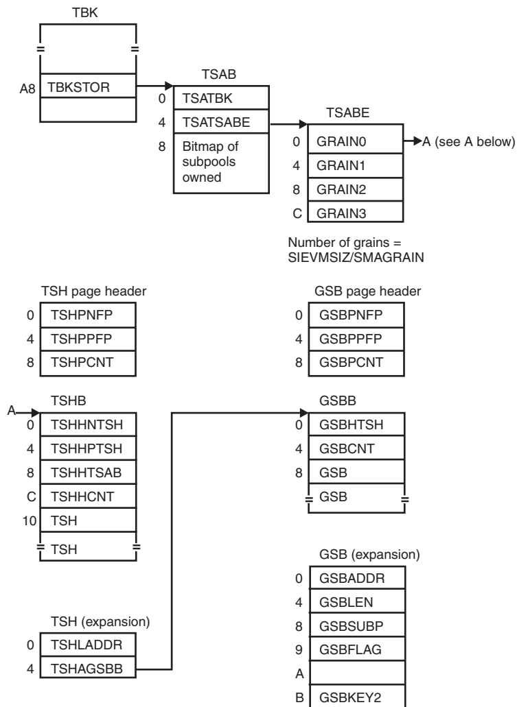
Figure 11. TSHB and GSBB Control Blocks
